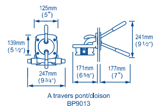
A travers pont/cloison BP9013
